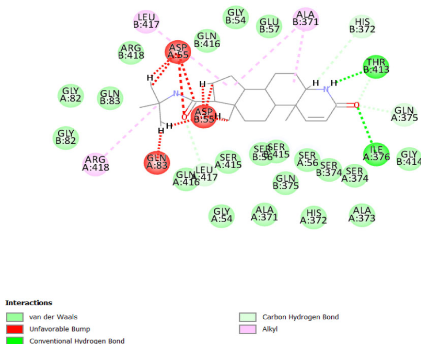
Fig. (S1). Interactions of finasteride with ALP.
