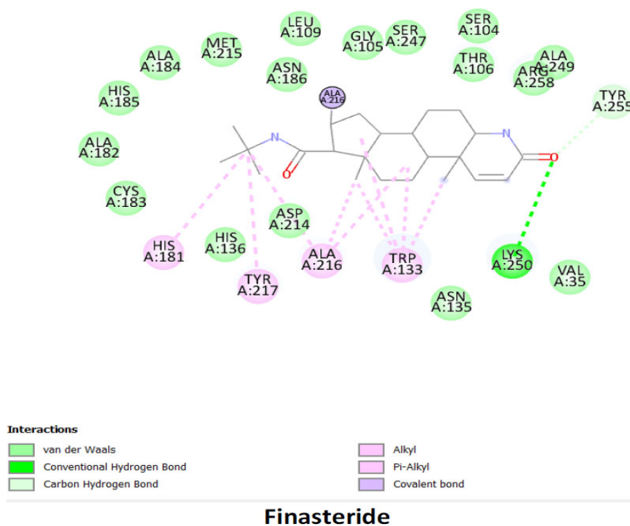
Fig. (S2). Interactions of finasteride with AST.
