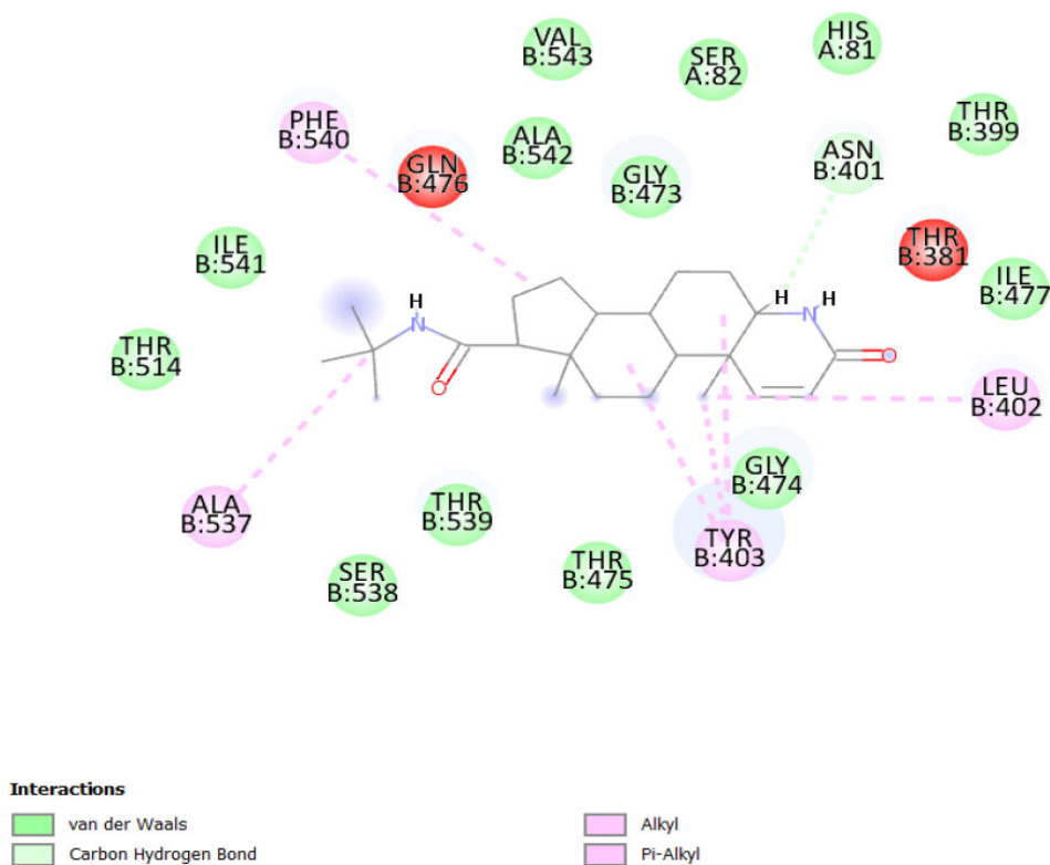
Fig. (S3). 2D interactions of finasteride with GGT.
